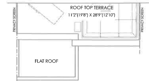
PARTIAL ROOF TOP TERRACE ELEV. 'C'
