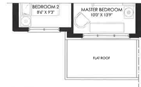
PARTIAL THIRD FLOOR PLAN & THIRD FLOOR FLEX PLAN ELEV. 'G' WITH ROOF TOP TERRACE
