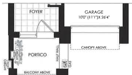
PARTIAL GROUND FLOOR PLAN ELEV. 'C'
