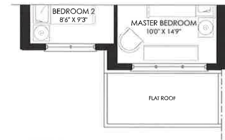
PARTIAL THIRD FLOOR PLAN & THIRD FLOOR FLEX PLAN ELEV. 'F' WITH ROOF TOP TERRACE
